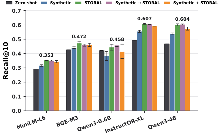
Figure 6: Recall@10 results for the fine-tuning experiments under the same inference-time configuration used in Figure 2. Results are averaged over three random seeds, with error bars denoting standard deviation.
