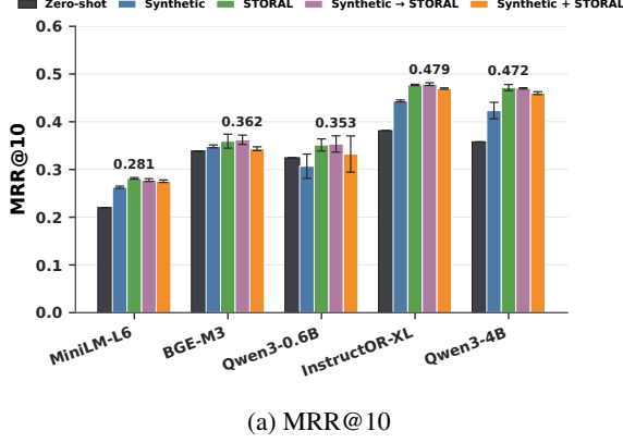
Figure 2: Fine-tuning results: Synthetic \rightarrow STORAL is curriculum learning, and Synthetic + STORAL is mixed training. Inference-time uses the summary+fable approach without instructions. Recall@10 is reported in Appendix M.
