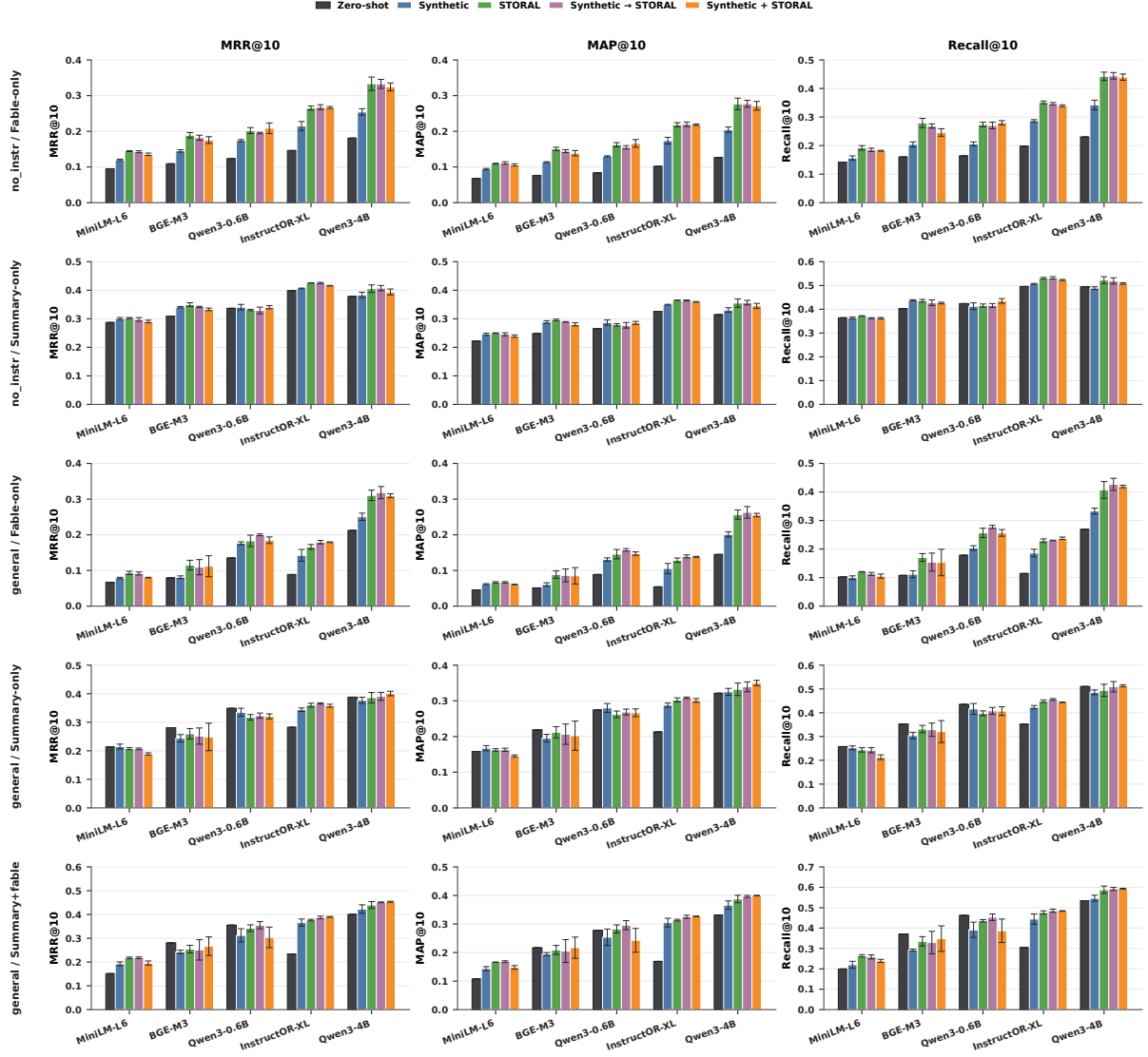
Figure 7: Fine-tuning results under additional fixed inference-time configurations using Gemini-generated direct_moral summaries. Rows correspond to document representation and query-instruction settings; columns report MRR@10, MAP@10, and Recall@10. The main paper fine-tuning figure reports the best fixed configuration, while this appendix figure shows complementary configurations.
